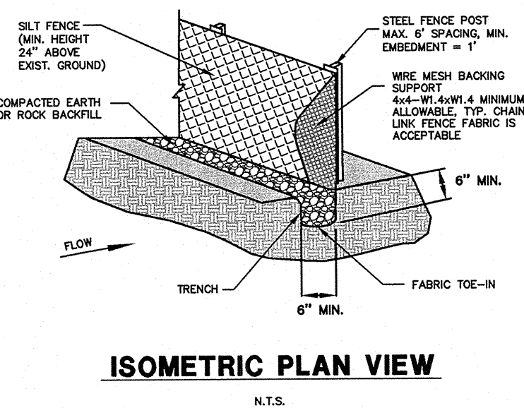
Schematic of a Silt Fence Installation (NCTCOG, 1993c)
