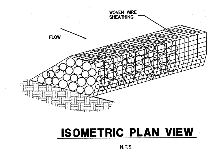
Schematic Diagram of a Rock Berm (NCTCOG, 1993)
